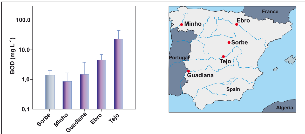
Figure 20. BOD (in \text{mg L}^{-1} ) at one baseline (Sorbe River) and four impact (Minho, Guadiana, Ebro and Tejo Rivers) monitoring stations in Spain. Data are mean \pm 1 standard deviation.
