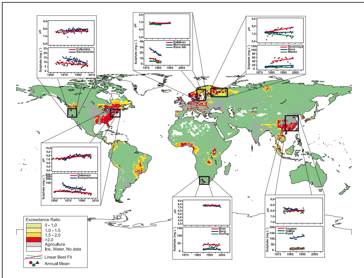
Figure 36. Trends in pH and sulphate concentrations in rivers around the world are overlayed onto a map showing sensitivity of an area to acidification. Sensitivity is measured as an exceedance ratio, which is the ratio of net acid deposition to critical load for an area, where critical load is a function of the acid buffering capacity of soils. Exceedance ratios greater than one indicate areas that are sensitive to acid deposition (Bouwman et al. , 2002). Note the general decreases in instream sulphate concentrations in the United States and Sweden, compared to increases in China and Russia. There was very little change in pH and sulphate concentrations in South Africa, which is considered at relatively low risk of acidification based on exceedance ratios. Changes in pH do not always parallel changes in sulphate concentrations, likely due to effects of other acidifying chemicals such as nitrates.
