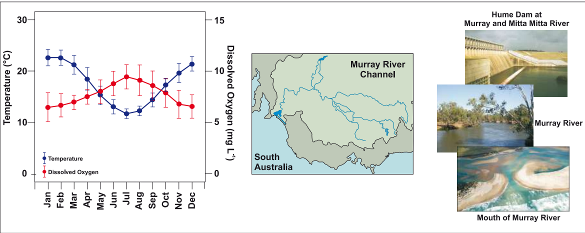
Figure 3. Seasonal patterns in dissolved oxygen and temperature in the Murray River, Australia. Data are monthly means \pm 1 standard deviation. Note that peaks in water temperature coincide with dissolved oxygen minima over the course of a year.
