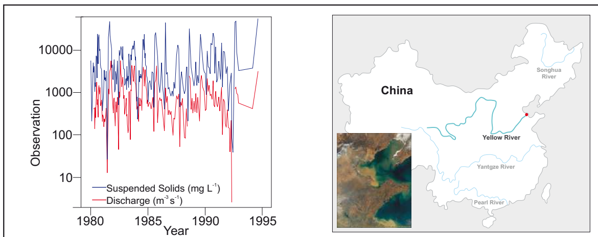
Figure 8. Suspended solids and instantaneous discharge measured in the Yellow River, China, at Lijin, approximately 80 km from the mouth of the river. Note how closely suspended solids concentrations track instantaneous discharge over time.
