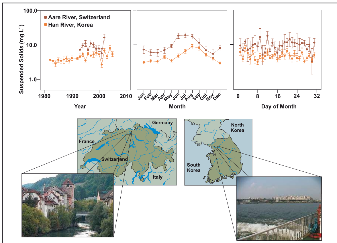
Figure 26. Temporal trends in suspended solids in the Aare River, Switzerland, and the Han River, Korea. Data are annual, monthly, and day of month means with standard deviations.
