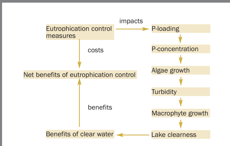
Figure 10. Model lay out (see text for explanation).
