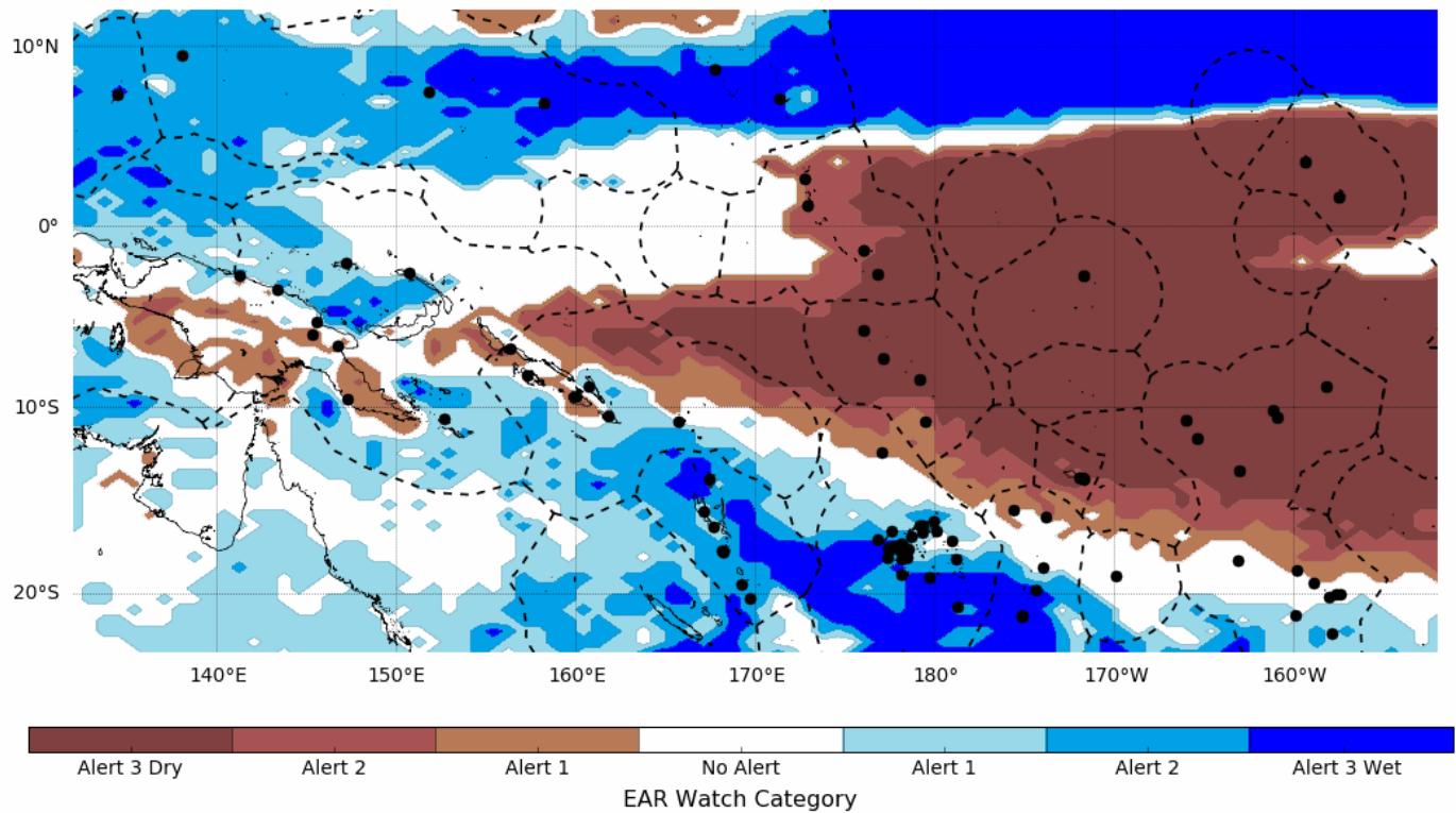
EAR Watch Categorical forecast for February 2022
